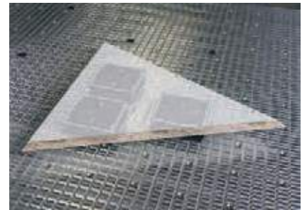
Vacuum clamp Vacuum clamping elements for insertion in the grooves of the Matrix table
