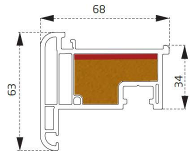
PDR1360BY Stümp Profili Stump Profile
