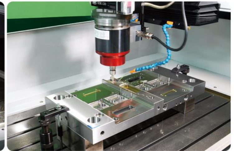
精密塑膠模座加工 Housing of high sophisticated plastic mold
