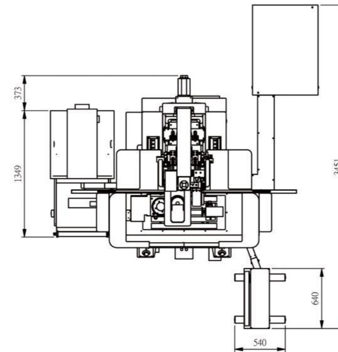
JG-510GC 內齒輪研磨機
