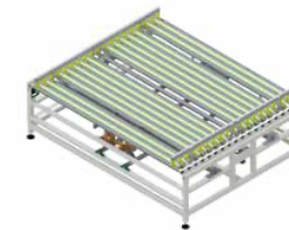
ET-ALGN-R Automatic Centralizing and Aligning Conveyor
