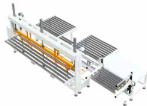
MSF-200 Semi Auto Tricot Inner Cover Filling and Sealing Machine
