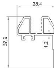
SINGLE GLASS ESPAGNOLETTE LOCK CONJUGATE PROFILE 313-2
