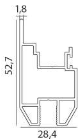
SINGLE GLASS ESPAGNOLETTE LOCK PROFILE 313-1
