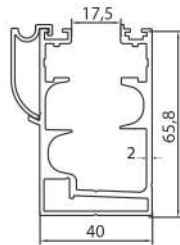
CASE PROFILE WITH RAIN CHANNEL 101-2
