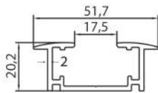
SLIM CASE PROFILE 103
