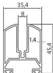
SQUARE BASE PROFILE 306-8 306-10
