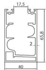
CASE PROFILE WITH GASKET 102
