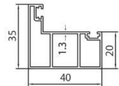
SIDE MAST PROFILE (8-10MM) 308
