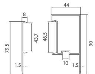
CASE ADJUSTMENT PROFILE 104
