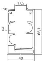
CASE PROFILE WITH DROPPER 101
