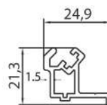
AURA 135° ANGLE PROFILE 110
