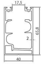
CASE PROFILE WITH GASKET 102
