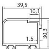
AURA 90° CORNER PROFILE 111
