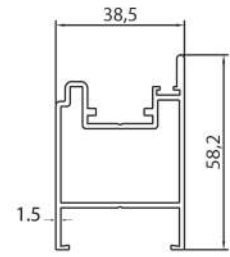
AURA STEM-LOCK PROFILE 113
