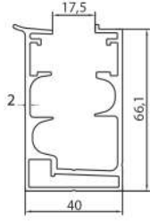
CASE PROFILE WITH DROPPER 101
