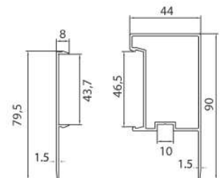
CASE ADJUSTMENT PROFILE 104
