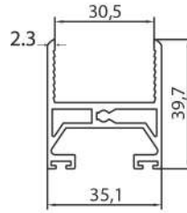
AURA BASE PROFILE 106
