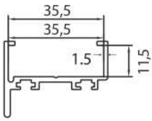
AURA LATH PROFILE 109
