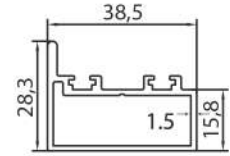
AURA SIDE MAST PROFILE 108
