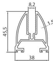
VISTA BASE PROFILE 406-8 406-10
