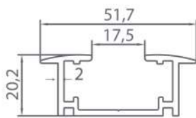
SLIM CASE PROFILE 103
