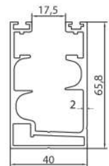
CASE PROFILE WITH GASKET 102
