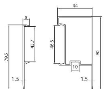
CASE ADJUSTMENT PROFILE 104
