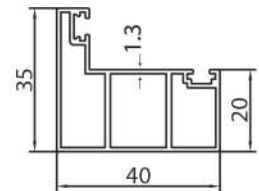
SIDE MAST PROFILE (8-10MM) 308
