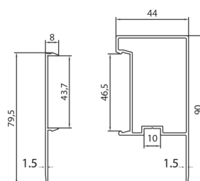
CASE ADJUSTMENT PROFILE 104
