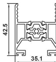
AURA-PLUS BASE PROFILE 206
