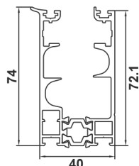
AURA-PLUS CASE PROFILE 201
