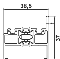
AURA-PLUS LATH PROFILE 209
