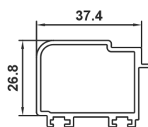
AURA-PLUS 90° CORNER PROFILE 211
