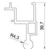
GIO-MATIC LOWER LEAF HINGE PROFILE 712 (3800 gr - 7 mt.)
