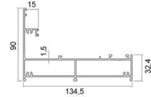
GIO-MATIC LOWER-UPPER CASE PROFILE 702 (11400 gr - 5.8 mt.)
