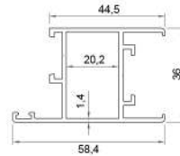
GIO-MATIC LEAF PROFILE 703 (5400 gr - 7 mt.)
