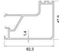
GIO-MATIC FIRST CHANNEL PROFILE 707 (4900 gr - 5.8 mt.)
