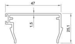
GIO-MATIC SECOND CHANNEL PROFILE 708 (2600 gr - 5.8 mt.)
