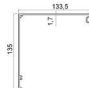
GIO-MATIC MOTOR ENCLOSURE PROFILE 711 (10600 gr - 7 mt.)
