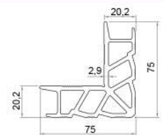
GIO-MATIC MITER PROFILE 715 (8200 gr - 3 mt.)
