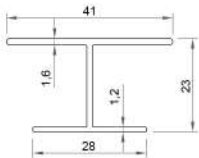
GIO-MATIC MOVABLE HIDING COVER PROFILE 709 (2100 gr - 5.8 mt.)
