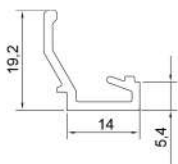
GIO-PLUS GLASS ADAPTER PROFILE 616 (2600 gr / 7.0 mt.)
