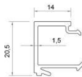
GIO-MATIC GLASS ADAPTER PROFILE 713 (1600 gr - 7 mt.)
