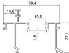
GIO-MATIC SIDE MAST ADAPTER PROFILE 706 (5100 gr - 5.8 mt.)
