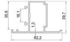
GIO-MATIC FIRST LEAF ADAPTER PROFILE 704 (3800 gr - 5.8 mt.)
