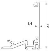
GIO-MATIC CLAMP PROFILE 705 (3700 gr - 7 mt.)
