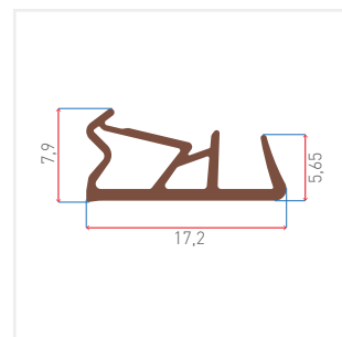
Technical Drawing
