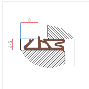
Application Drawing
