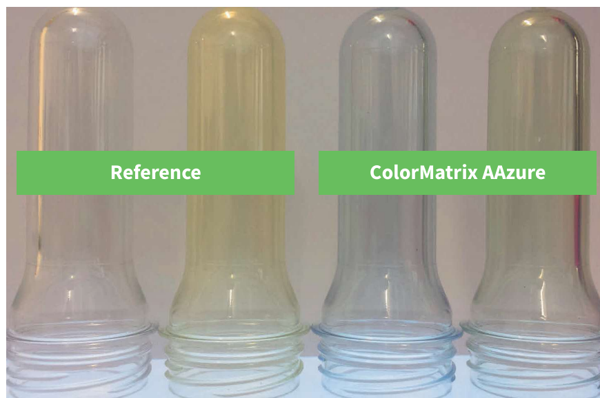
Impact of 5 Melt Heat Histories on Preform Color
