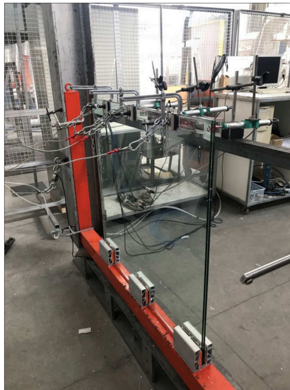
Photograph of the item after the horizontal static loading test
