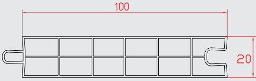
100mm LAMBRİ (Two Chamber Panel Profile)
