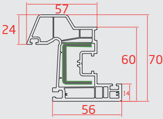
DAMLALIKLI KANAT (Self Drainage Sash Profile)
