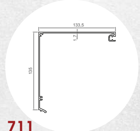
711 Gio-Matic Motor Kutu Profil Gio-Matic Engine Box Profile (10600 gr - 7 mt.)
