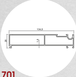
701 Gio-Matic Alt-Üst Kasa Profil Gio-Matic Lower-Upper Case Profile (10000 gr - 7 mt.)
