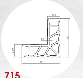
715 Gio-Matic Köşe Gönye Profil Gio-Matic Corner Profile (3100 gr - 3 mt.)
