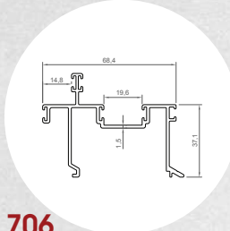
706 Gio-Matic Yan Dikme Adaptör Profil Gio-Matic Side Mast Adaptor Profile (4400 gr - 5 mt.)
