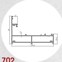
702 Gio-Matic Yan Dikme Kasa Profil Gio-Matic Side Mast Profile (9600 gr - 5 mt.)
