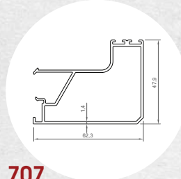
707 Gio-Matic Birinci Kanal Profil Gio-Matic First Channel Profile (4200 gr - 5 mt.)
