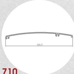
710 Gio-Matic Kapak Profil Gio-Matic Cover Profile (4200 gr - 7 mt.)
