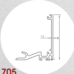
705 Gio-Matic Kenet Profil Gio-Matic Clamp "Leaf" Profile (3700 gr - 7 mt.)
