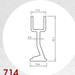
714 Gio-Matic Zincir Profil Gio-Matic Chain Profile (4300 gr - 5 mt.)
