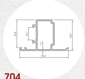
704 Gio-Matic İlk Kanat Adaptör Profil Gio-Matic First Leaf Adaptor Profile (3200 gr - 5 mt.)
