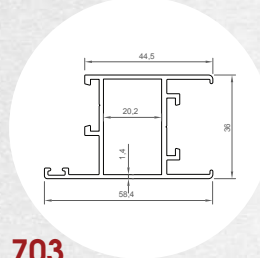
703 Gio-Matic Kanat Profil Gio-Matic Leaf Profile (5400 gr - 7 mt.)
