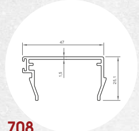
708 Gio-Matic İkinci Kanal Profil Gio-Matic Second Channel Profile (2200 gr - 5 mt.)
