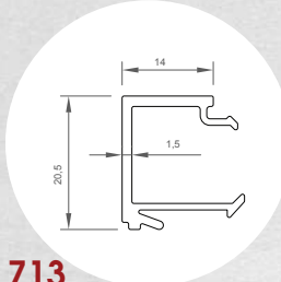
713 Gio-Matic Cam Çıta Profil Gio-Matic Glass Adaptor Profile (1600 gr - 7 mt.)
