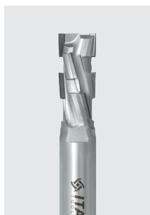
PCD router bit Z2+1 - DTN series
